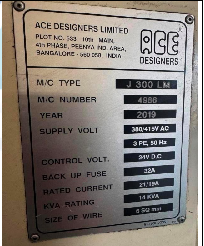
View of Ace CNC Lathe Model: J 300LM, Sr. No. 4986 Installed at Unit-3
