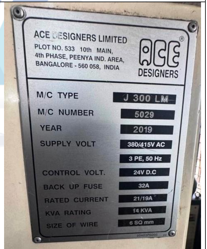
Ace CNC Lathe Model: J 300LM, Sr. No. 5029 Installed at Unit-3
