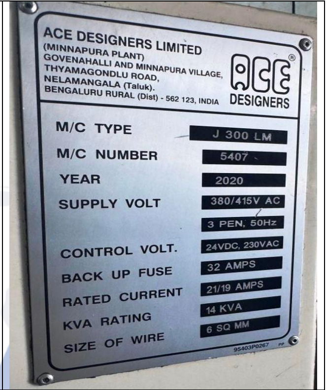
View of Ace CNC Lathe Model: J 300LM, Sr. No. 5407 Installed at Unit-3
