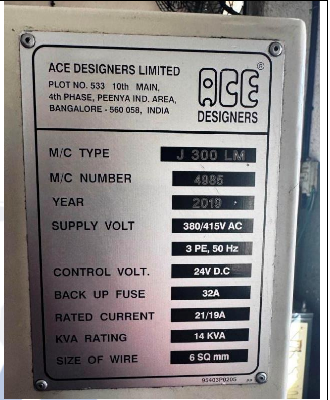
View of Ace CNC Lathe Model: J 300LM, Sr. No. 4985 Installed at Unit-3
