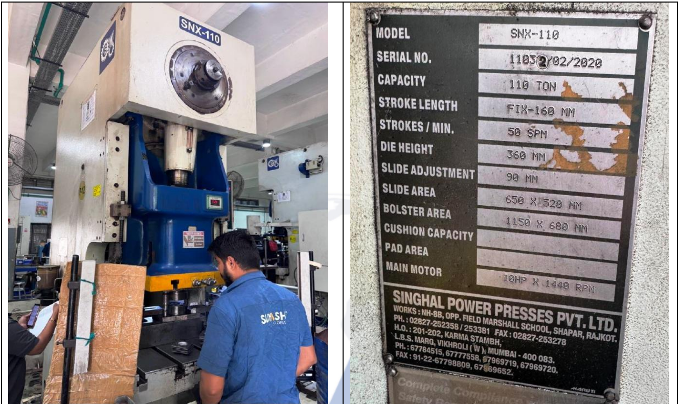
View of Sewcross Shaft Geared Power Press Complete with Standard Accessories, Model SNX - 110T (SG), Sr. No. 11032/02/2020 Installed at Unit-4
