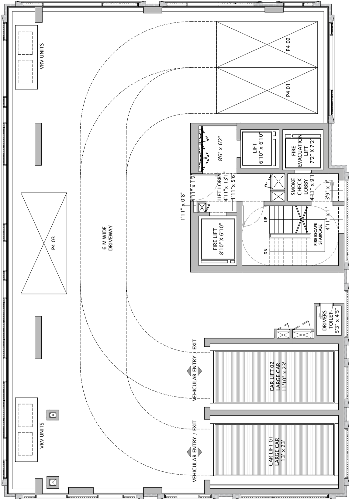
P4 LEVEL PODIUM PLAN
