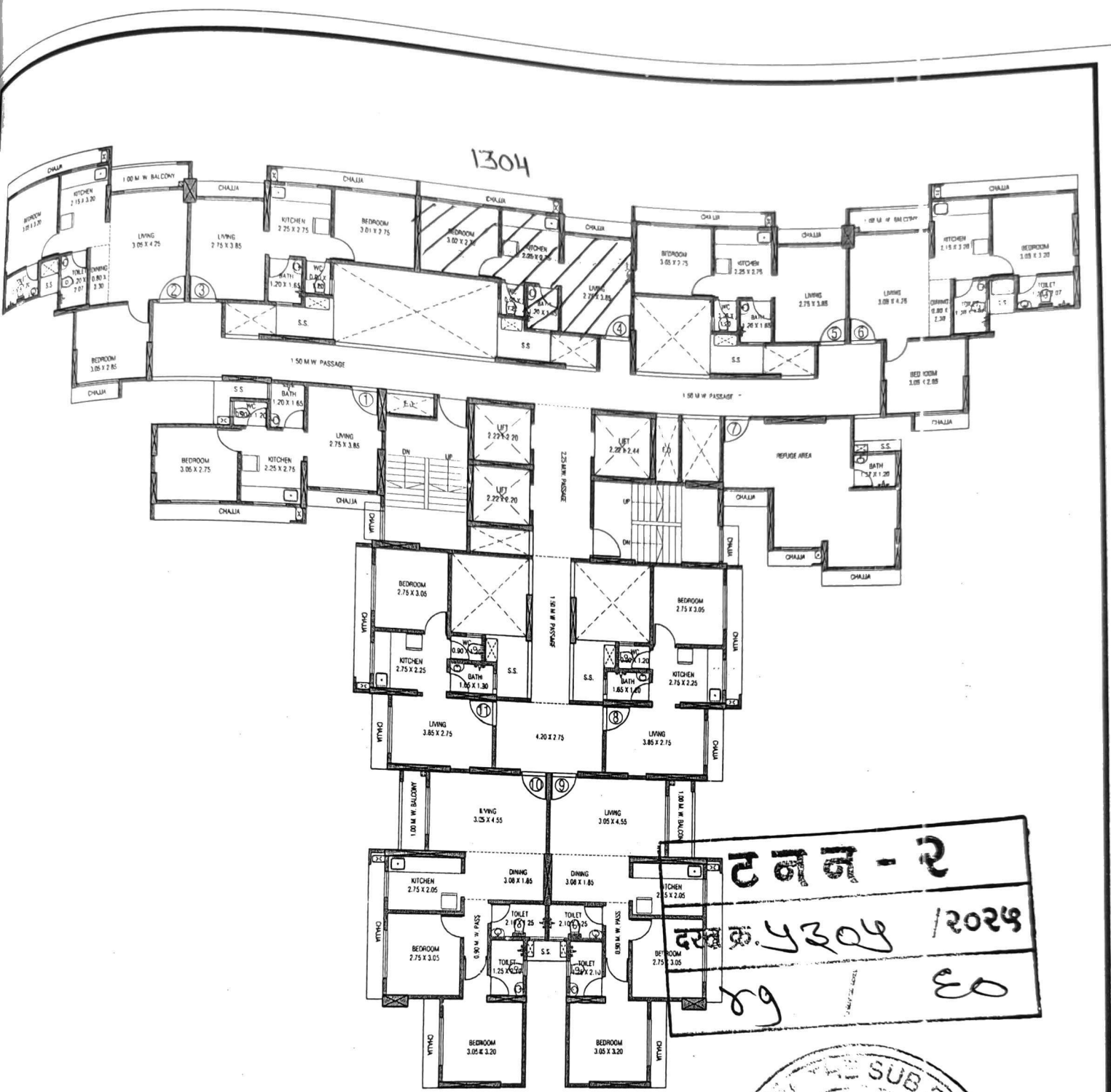
REFUGE FLOOR PLAN (8TH, 13TH & 18th)
