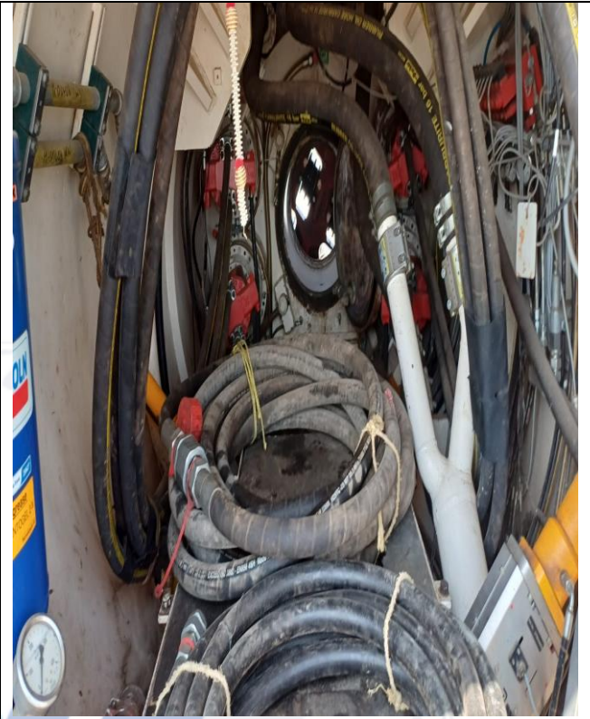
View of Used Tunneling Machine (M-406M AVN1 600T8, M-1332C)
