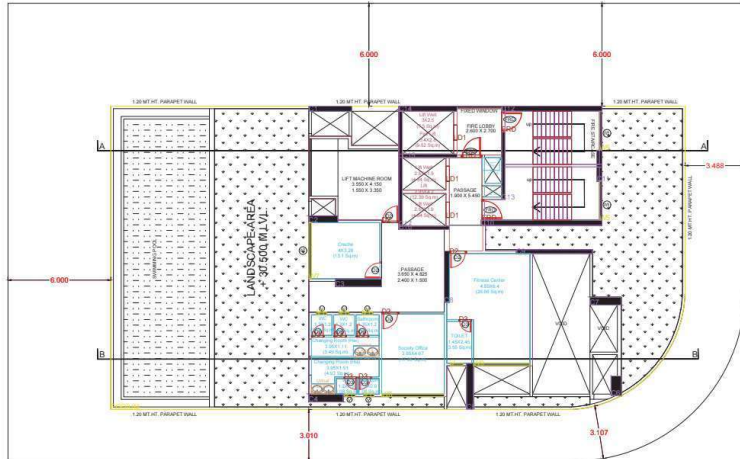
PODIUM LEVEL PLAN SCALE = 1:100
