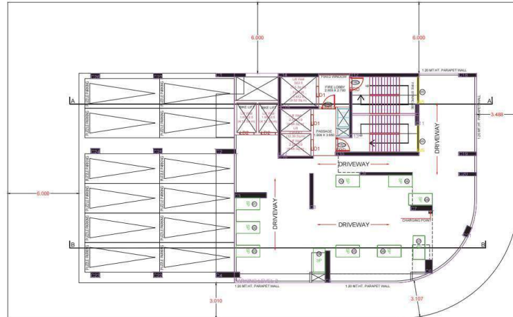
PARKING LEVEL - 2 PLAN SCALE = 1:100 TOTAL AVAILABLE PARKING = 1620 SQ M
