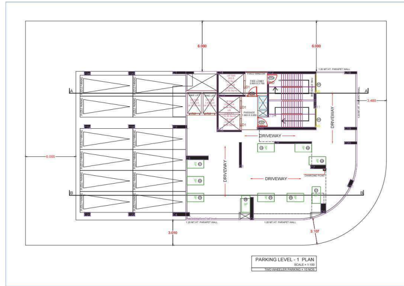
Parking Check As Per Multiplying Factor : 0.80
