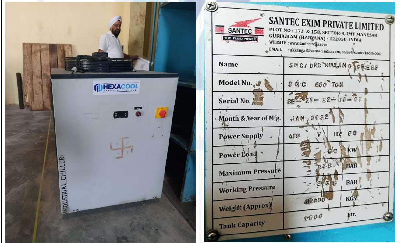
View of Santec make Hydraulic Moulding Press Model-SMC 600 Ton, Sr. No. SE-21-22-U5-09
