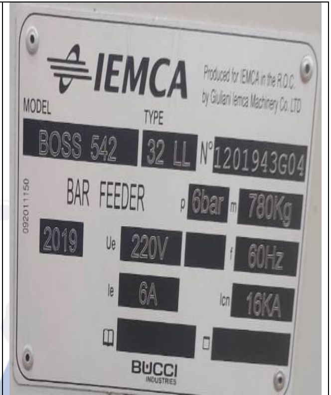
Bar Feeder, BOSS 542/32 - LL TYPE FOR NEXTURN SA 32 PYII
