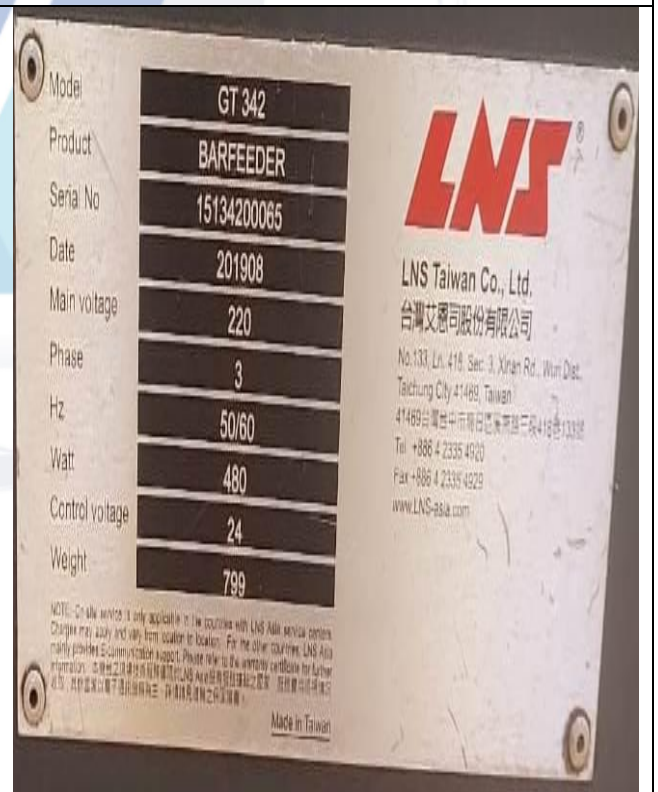
Automatic Bar Feeder, Model- GT 342, Length-3.2 Mtrs.
