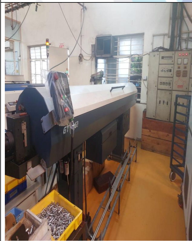
Automatic Bar Feeder, Model- GT 342, Length-3.2 Mtrs.
