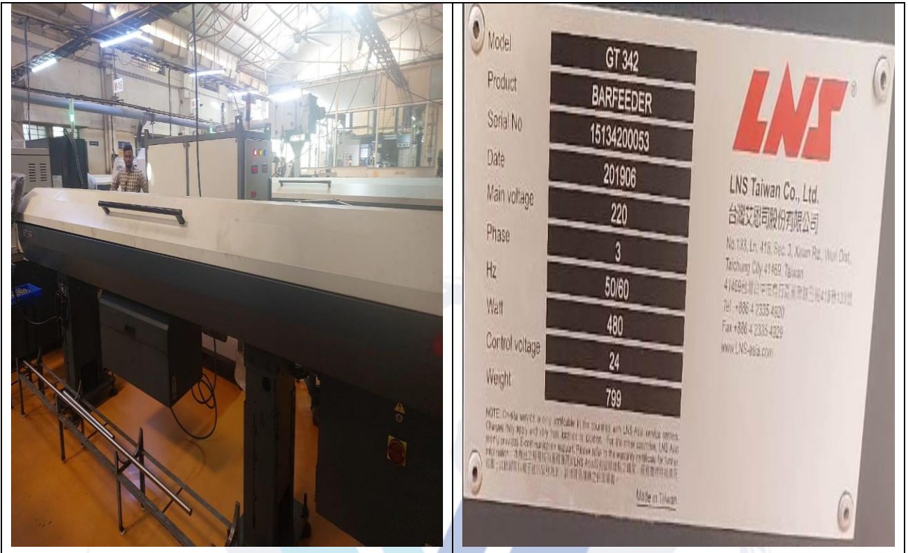
Automatic Bar Feeder, Model- GT 342, Length-3.2 Mtrs.
