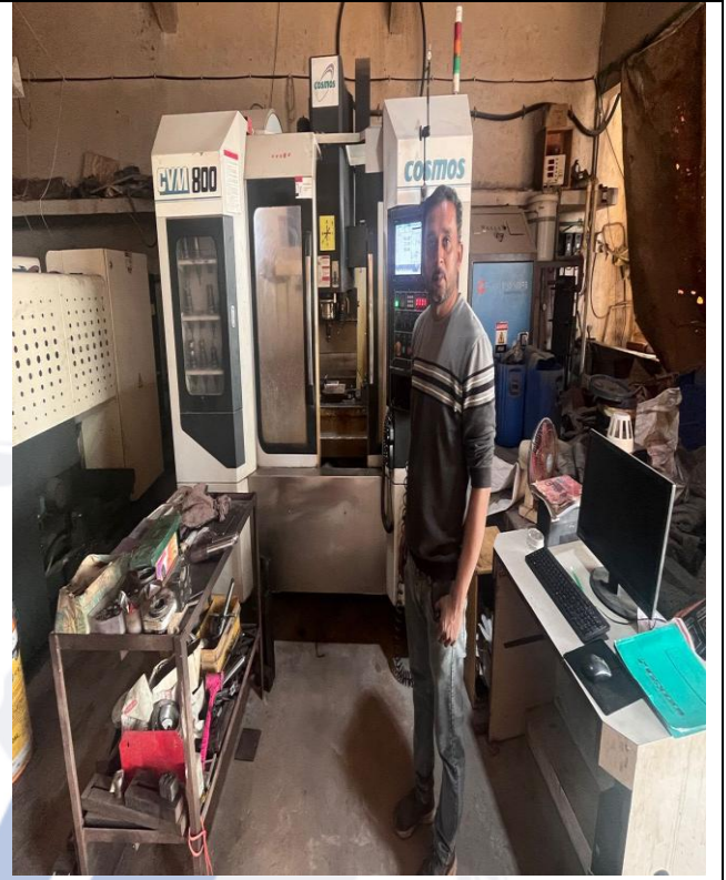
View of Cosmos Vertical Machining Centre, Model: CVM 800, Sr. No. 08 2339
