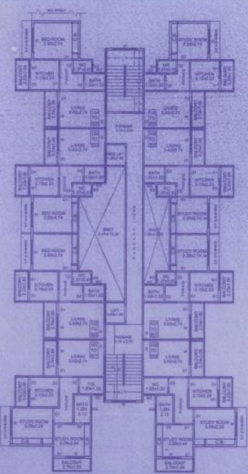
TYPICAL - 1ST-6TH FLOOR PLAN
