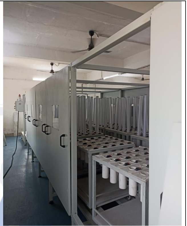
Ageing Line for LED Batten-Aging Capacity-850 Nos. , YOM-2024
