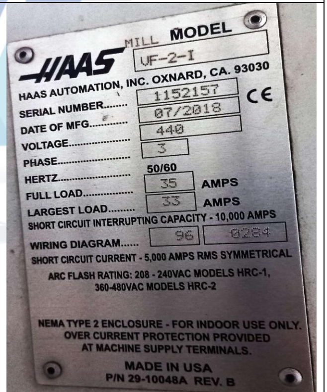
View of Vertical Machining Center, Model: - VF-2 I, Sr. No. 1152157, YOM-2018
