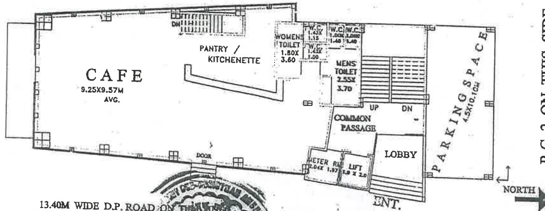
GROUND FLOOR PLAN FOR SAMARTHA ANNEXE WORKING DRG.
