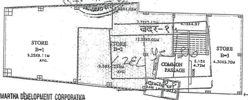
BESEMENT FLOOR PLAN FOR SAMARTHA ANNEXE WORKING DRG.
