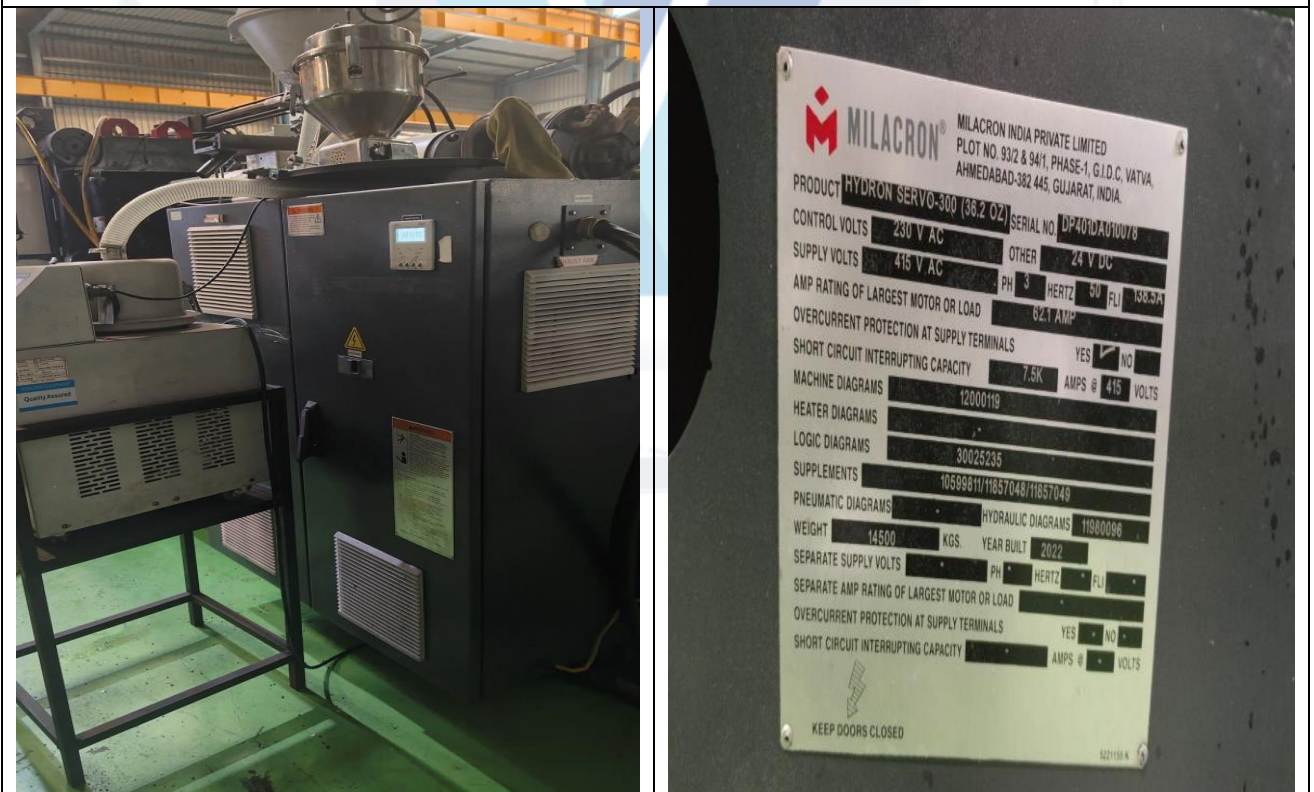
Injection Moulding Machine, Model-Hydron 300 Servo, Sr. No. DP401DA010078
