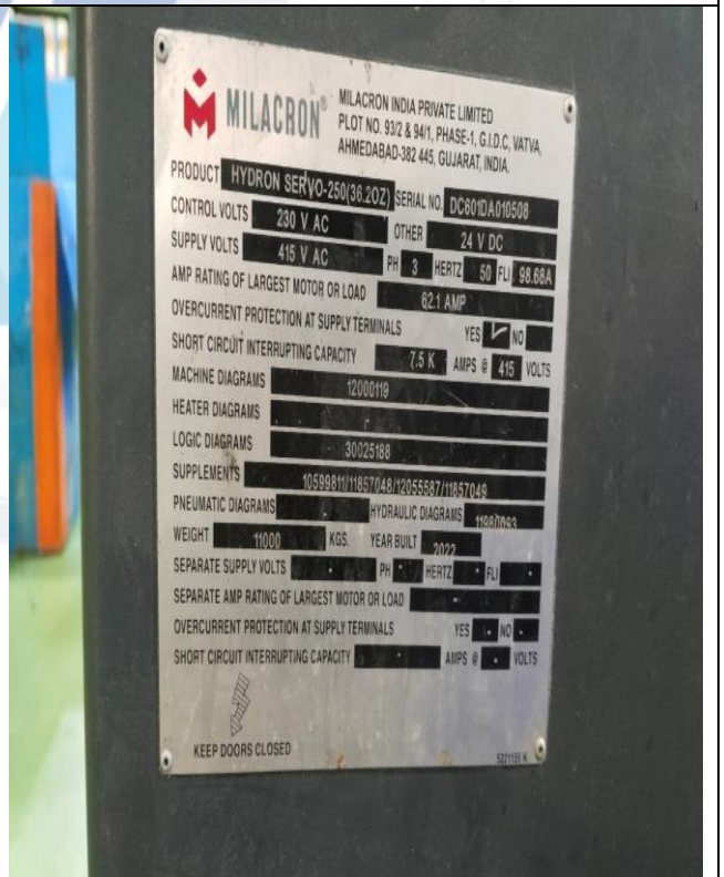
Injection Moulding Machine, Model-Hydron 250 Servo, Sr. No. DC601DA010508
