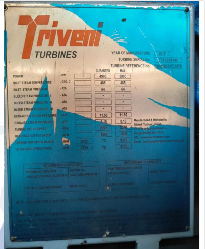
Name Plate of Turbine
