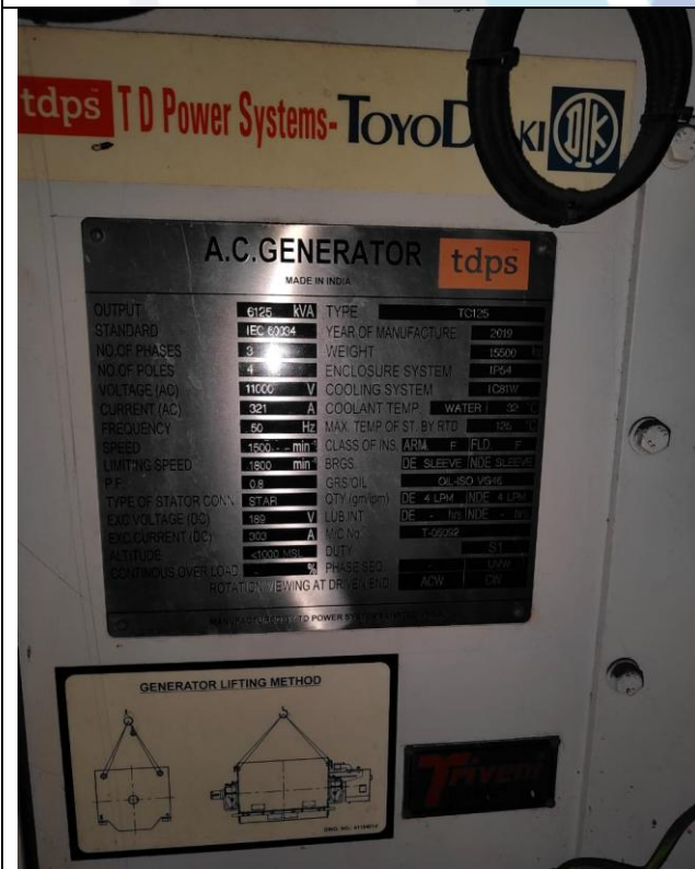
Name Plate of Generator
