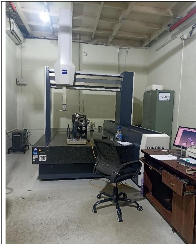
Carl Zeiss Make, 3D CNC Co-ordinate Measuring Machine, Model-CMM Contura
