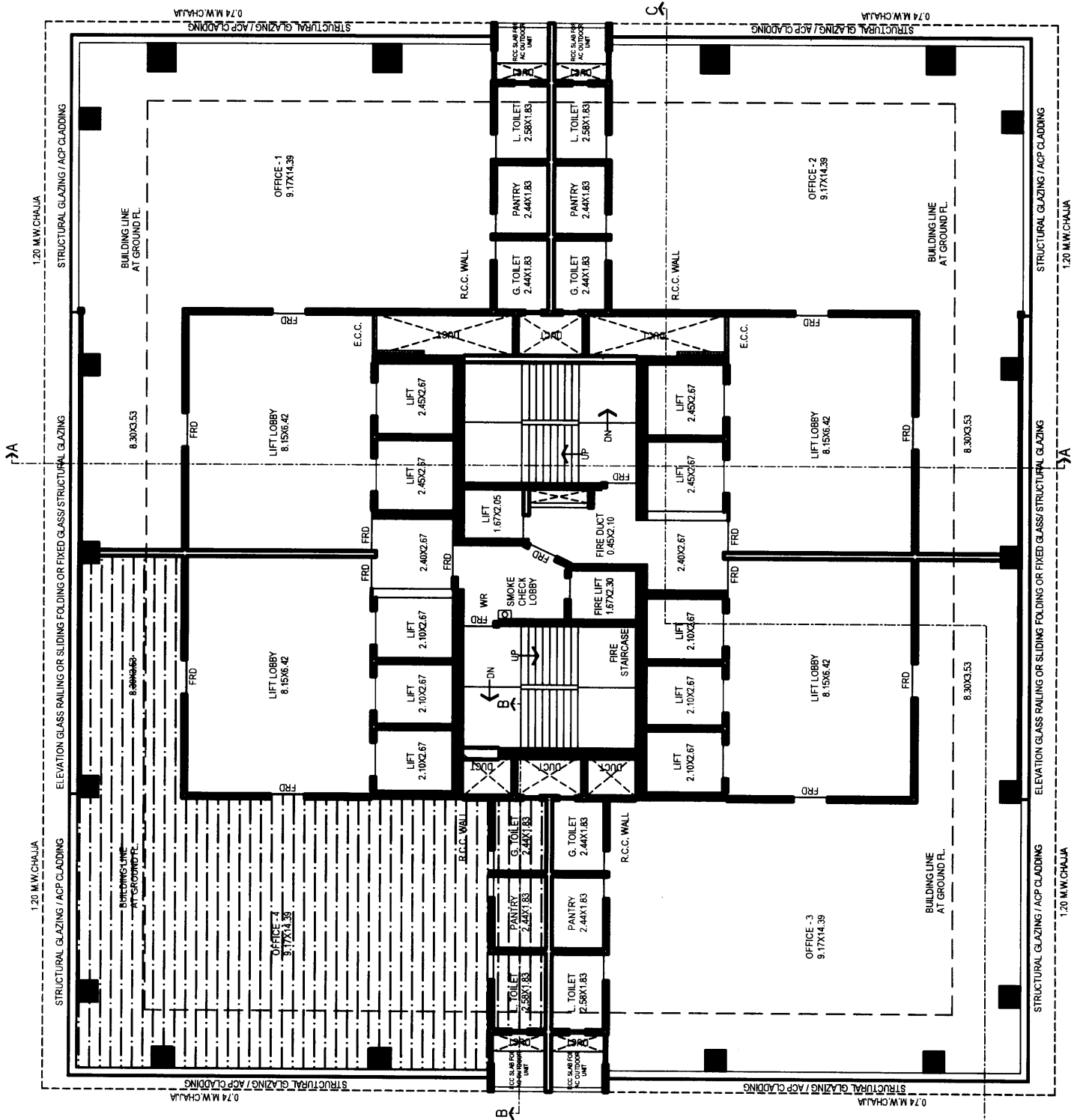
10th To 12th, 14th, 18th To 21st, 23rd To 26th FLOOR PLAN SCALE: 1:100
