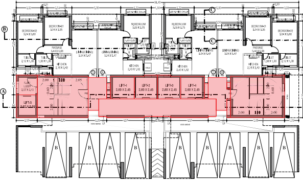
3rd & 4th FLOOR PLAN (WING-A-B) SCALE: 1:100
