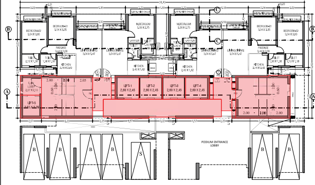
Sub-FLOOR PLAN (WING-A-B) SCALE: 1:100
