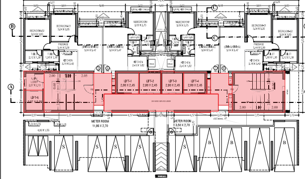
2nd FLOOR PLAN (WING-A-B) SCALE: 1:100
