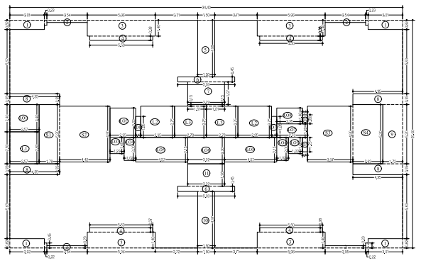
LINE AREA DIAGRAM FOR 6th to 7th, 9th to 14th, 16th to 21st, 23rd to 28th TYPICAL FLOOR (WING-A-B) SCALE: 1:100
