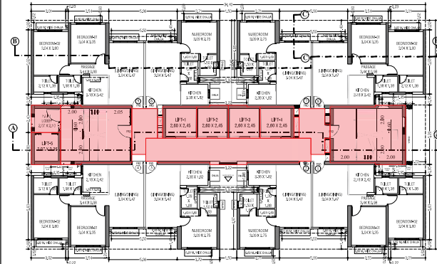
6th to 7th, 9th to 14th, 16th to 21st, 23rd to 28th TYPICAL FLOOR (WING-A-B) SCALE: 1:100
