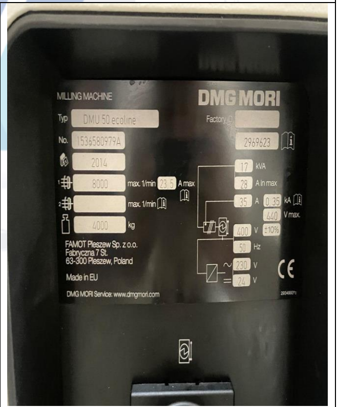
Universal Milling Machine, Model- DMU 50 Ecoline, Sr. No. 1536580979A
