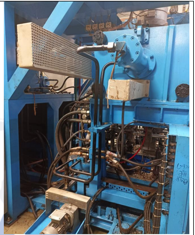
15 Ltr Single Station Blow Moulding Machine
