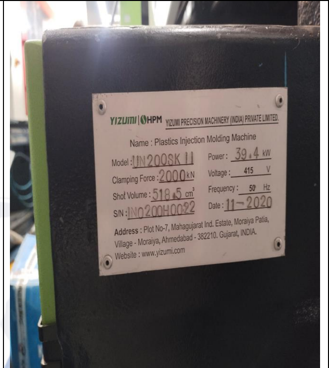
3 Platen Toggle Injection Moulding Machine, Locking Force-200 Ton, Screw Dia. 53 mm (Type-B), Sr. No. IN0200H0022
