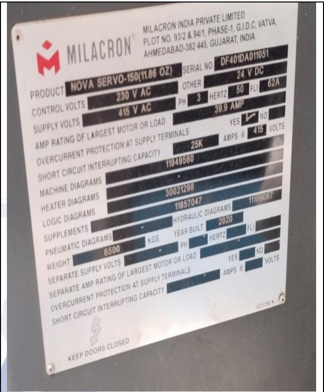
Injection Moulding Machine, Model- Nova 150 Servo, Sr. No. DF401DA011051
