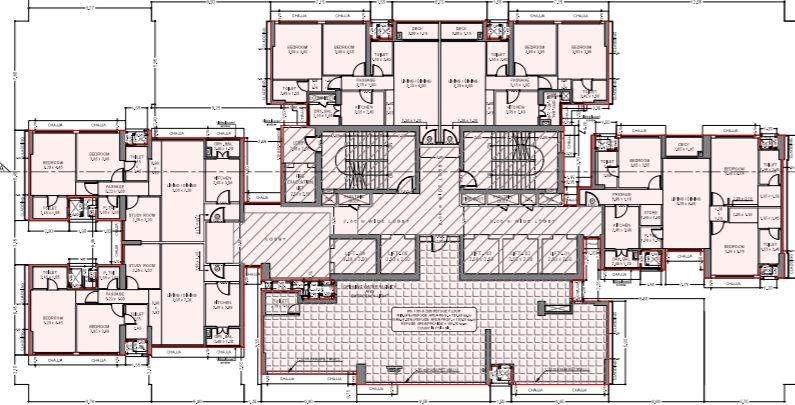
TYPICAL 6th, 13th & 20th REFUGE FLOOR PLAN
