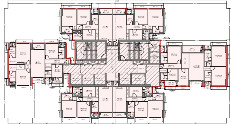
TYPICAL 2nd to 5th, 7th to 12th, 14th to 19th, 21st to 26th FLOOR PLAN
