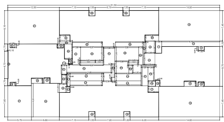
AREA DIAGRAM FOR TYPICAL 2nd to 5th, 7th to 12th, 14th to 19th, 21st to 26th FLOOR
