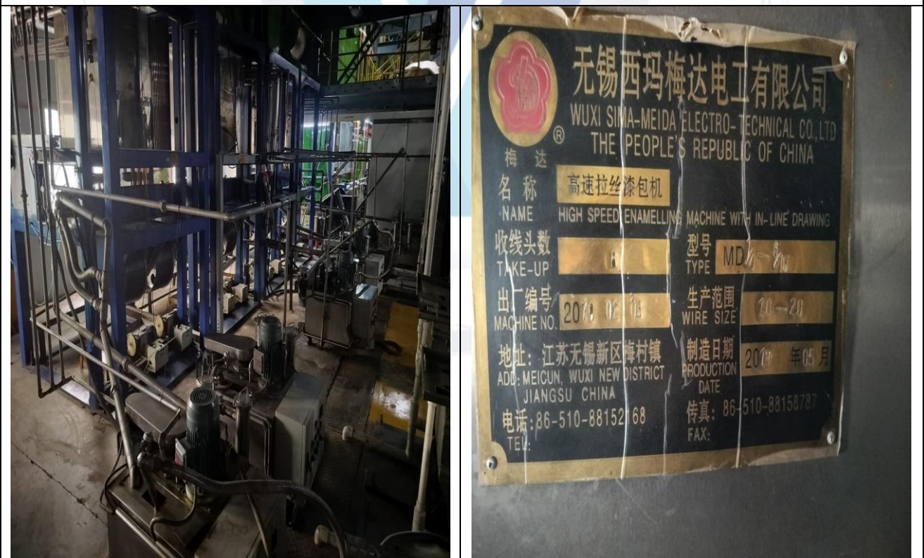
MDLI/8-8/16 Type Vertical High Speed Enamelling Machine
