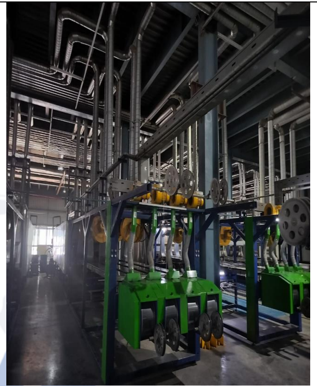
MD5/4-4/24F-2019 Type Horizontal High Speed Enamelling Machine
