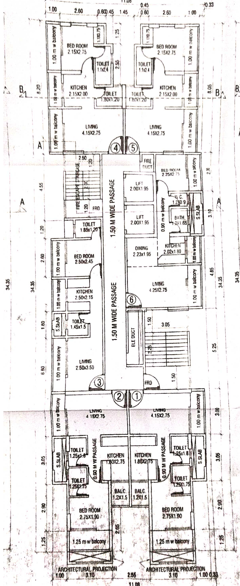
TYPICAL FLOOR PLAN WING-A SCALE 1:100 2ND TO 6TH & 8TH TO 10TH
