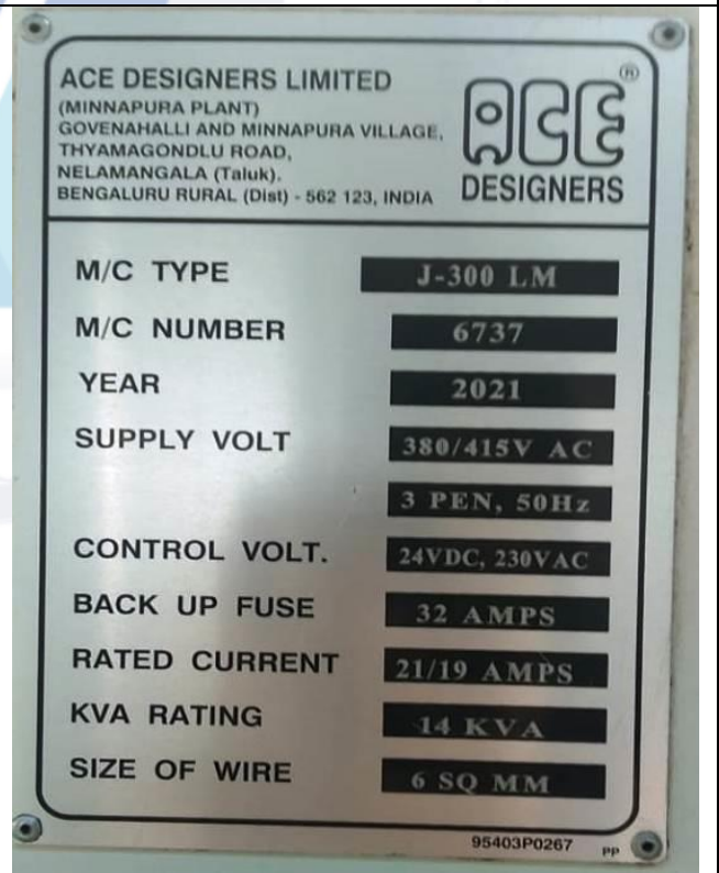
Ace CNC Lathe, Model- J 300 LM, Sr. No. 6737
