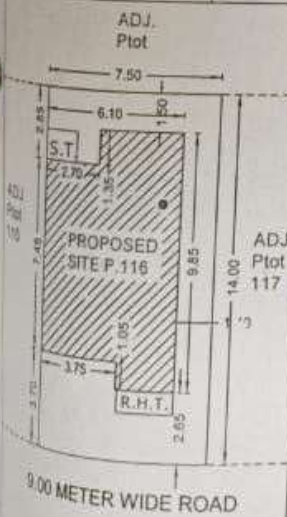
SITE PLAN SCALE = 1:250
