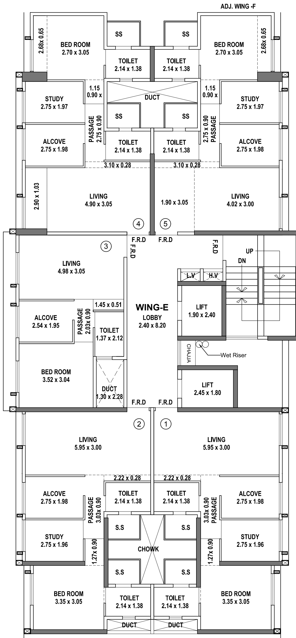
(WING - E ) TYPICAL FLOOR PLAN
