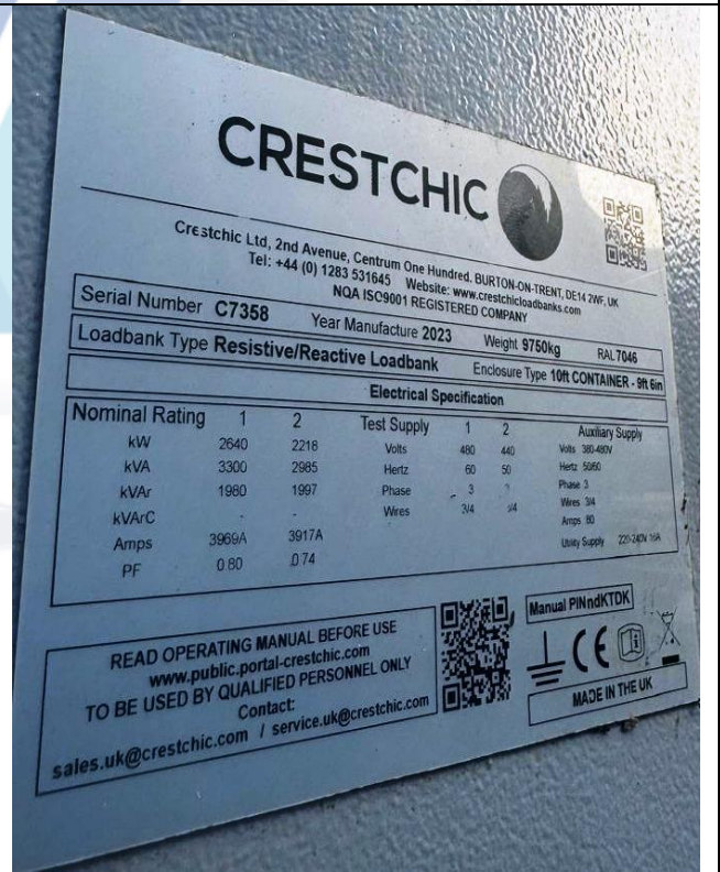
View of 3300 kVA Load Bank, Sr. No. C7358 at Location-2
