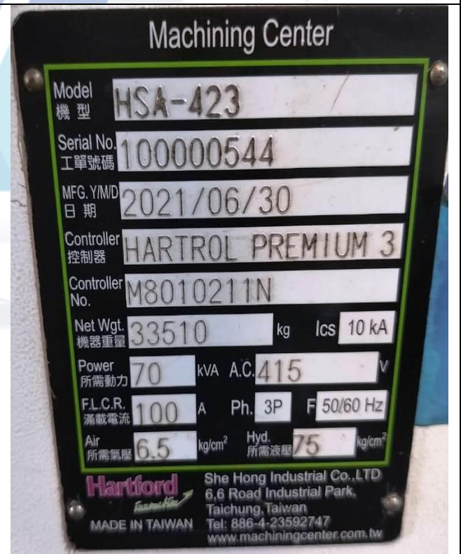
View of Hartford Brand Double Column Machining Centre, Sr. No. 100000544
