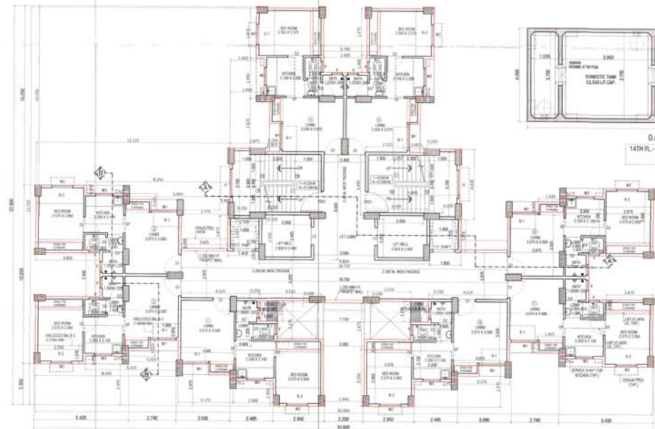
TYPICAL FLOOR PLAN EWS(R) (1st to 7th, 9th, 11th, 13th & 14th)
