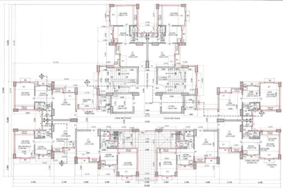
REFUGE FLOOR PLAN EWS(R) (8th, 10th & 12th fl.)
