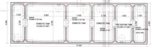
O.H. WATER TANK PLAN 14TH FL. - DOMESTIC 53,550 LIT. CAP. FIRE FIGHTING 20,000 LIT. CAP.
