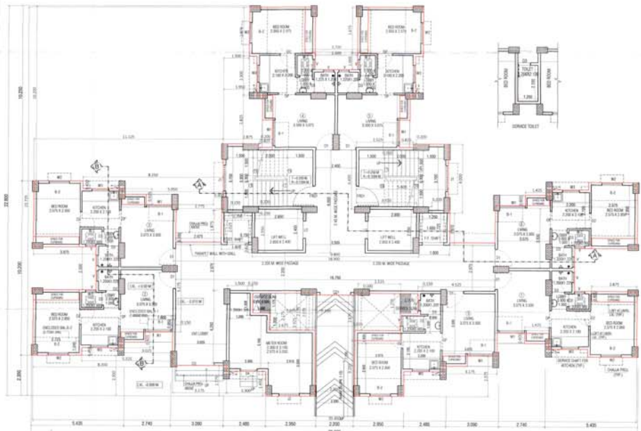
GROUND FLOOR PLAN EWS(R)
