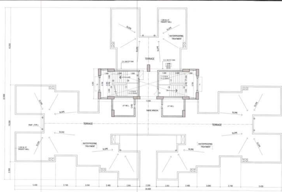
TERRACE FLOOR PLAN EWS(R)
