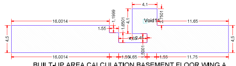
BUILT-UP AREA CALCULATION BASEMENT FLOOR WING A
