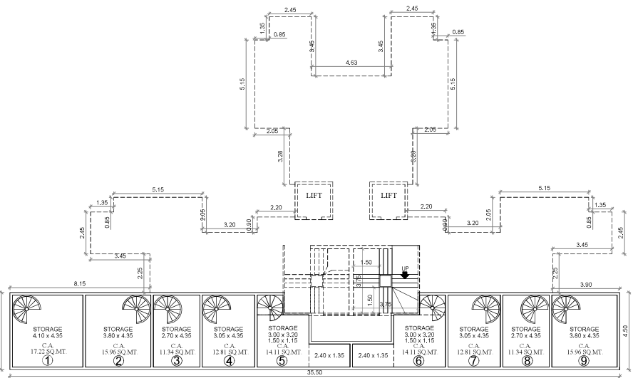
BASEMENT FLOOR PLAN WING A SCALE-1:100
