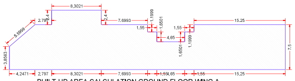
BUILT-UP AREA CALCULATION GROUND FLOOR WING A
