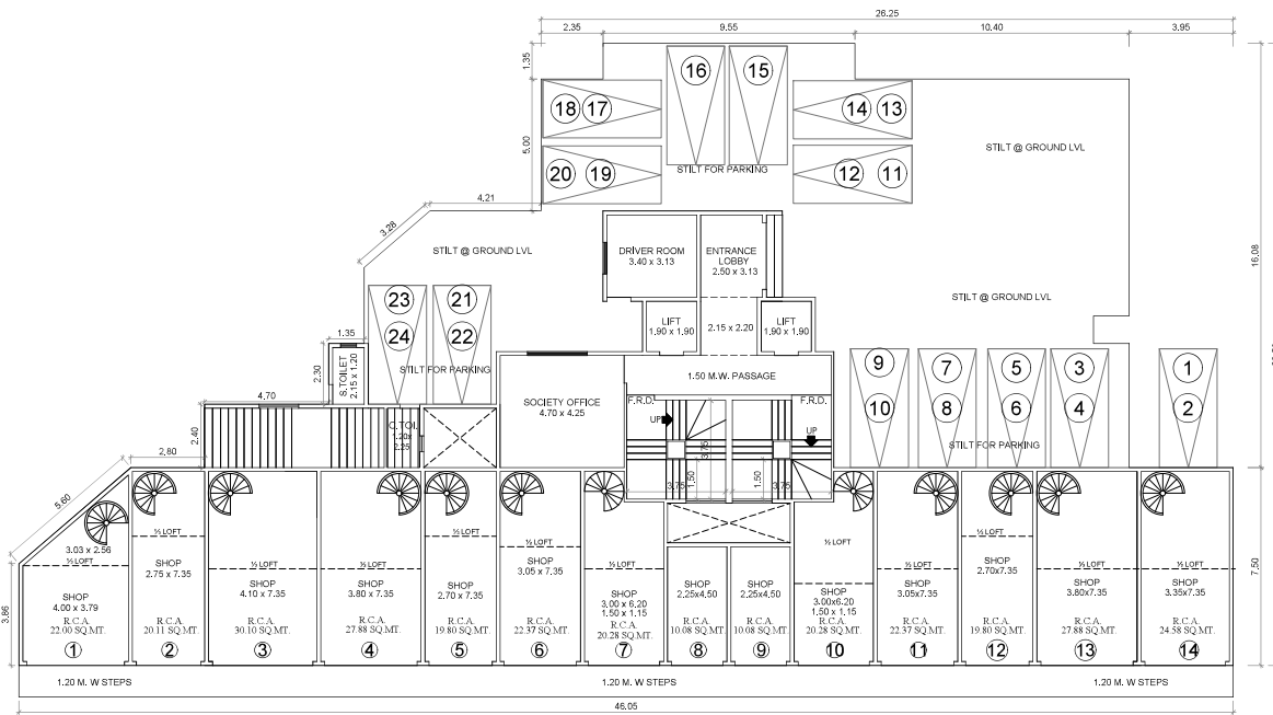
GROUND FLOOR PLAN WING A SCALE-1:100
