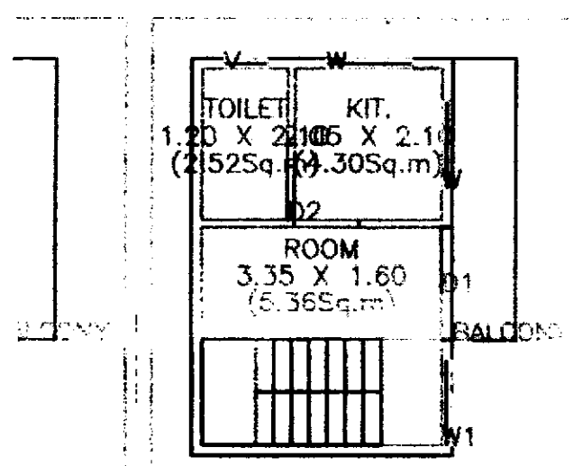
SECOND FLOOR PLAN (SCALE 1:100)
