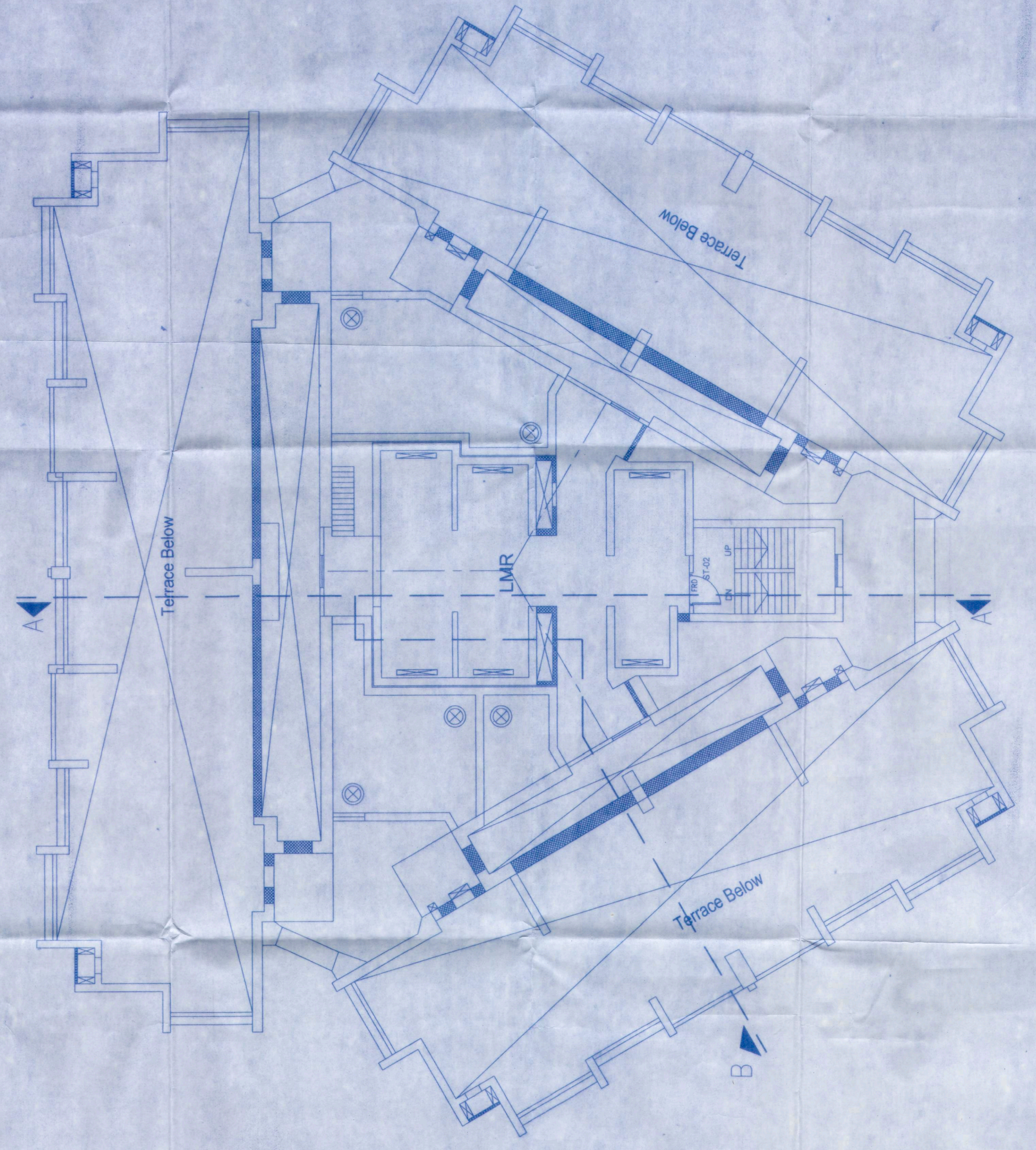
LMR LEVEL PLAN (TOWER-A) SCALE: 1:100
