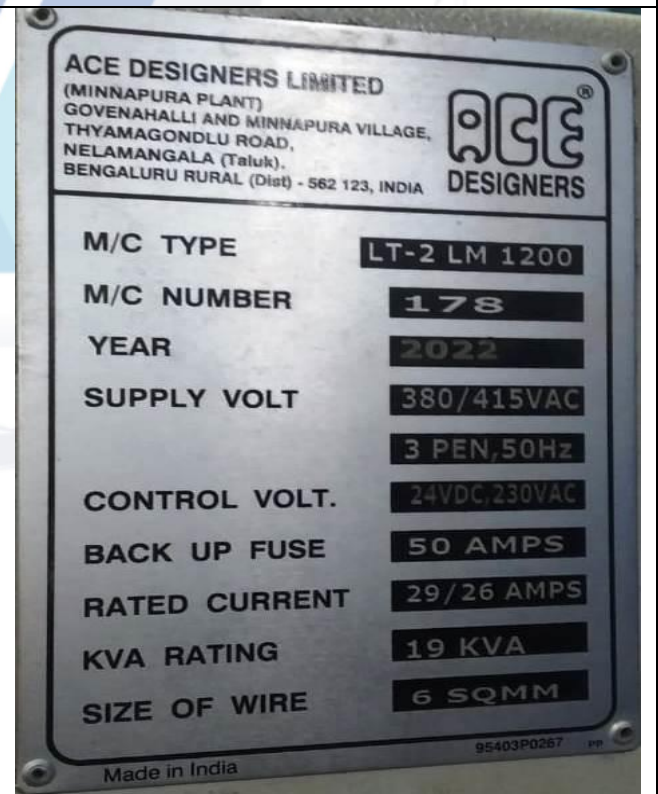
View of Ace CNC Lathe Model-LT 2 LM 1200, Sr. No.178
