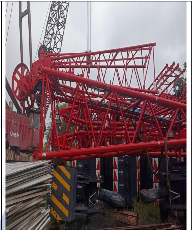
Super Lift Mast Boom at Panvel Workshop
