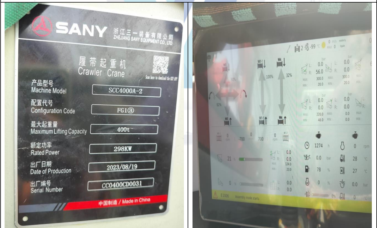
View of 400T Crawler Crane located at Kodinar Site
