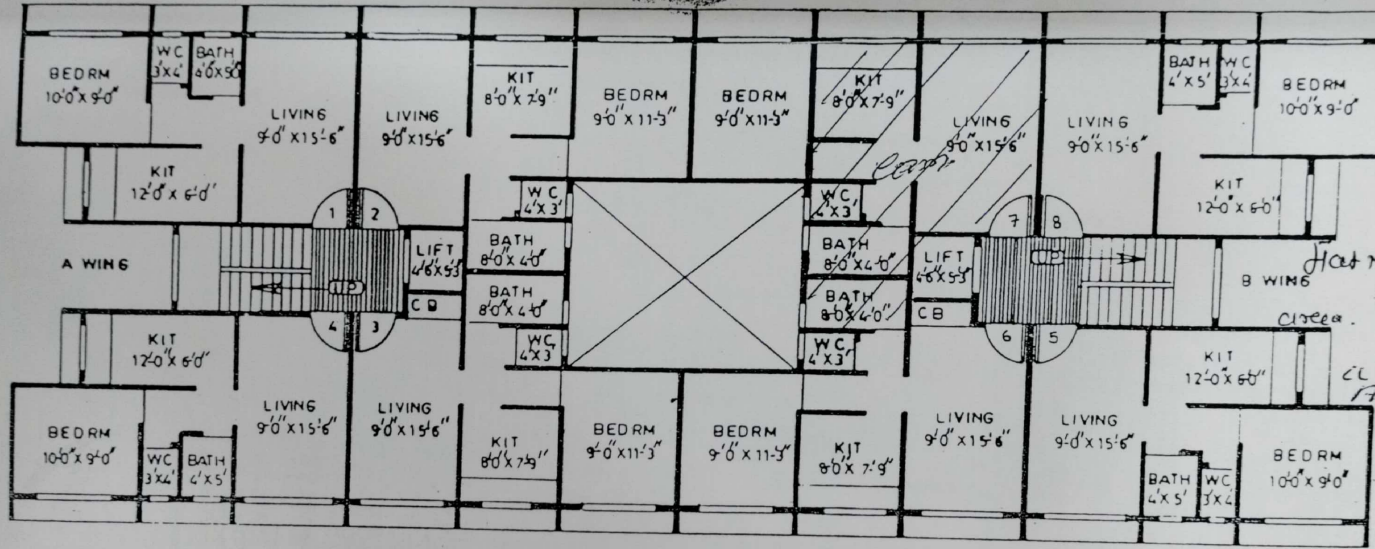
TYPICAL FLOOR PLAN 1ST TO 7TH FLR
