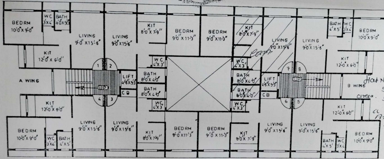
TYPICAL FLOOR PLAN 1ST TO 7TH FLR
