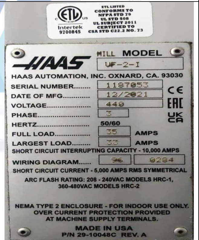
View of CNC Vertical Machining Centre, Model-VF-2-I, Sr. No. 1187053
