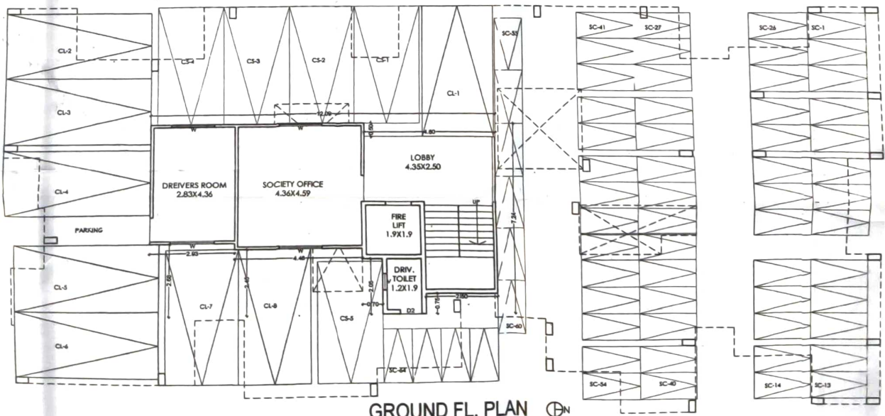
GROUND FL. PLAN
