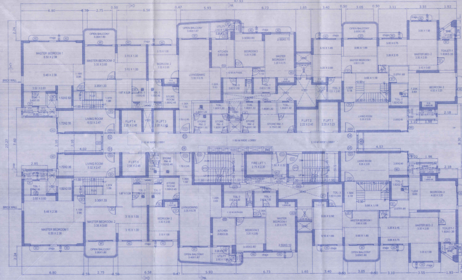
39TH (PENTHOUSE) FLOOR PLAN Scale - 1:100
