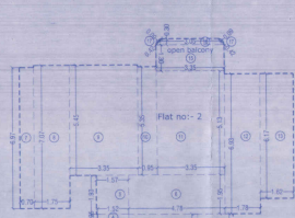
40th Floor Flat Area Diagram for Rera carpet (Flat no.2) SCALE - 1:100
