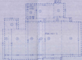
40th Floor Flat Area Diagram for Rera carpet (Flat no.1) SCALE - 1:100
