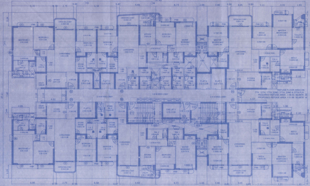
REFUGE FLOOR PLAN 12th, 17th, 22nd, 27th, 32nd & 37th floor Scale - 1:100
