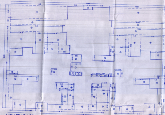
LINE AREA DIAGRAM FOR GROUND FLOOR PLAN SCALE: 1:100
