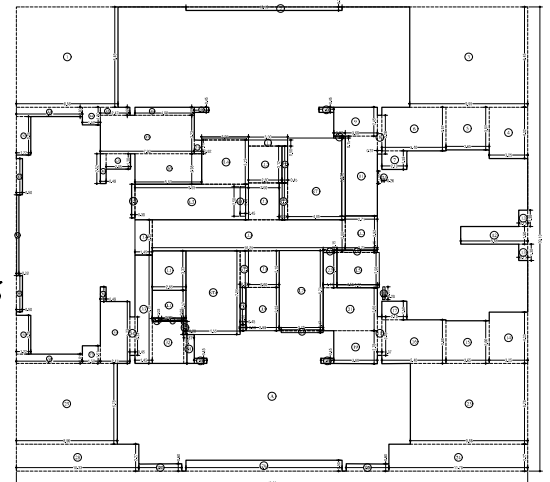
LINE AREA DIAGRAM FOR 30TH TO 35TH, 37TH TO 42ND, 44TH TO 47TH TYPICAL FLOOR PLAN (WING-4)
