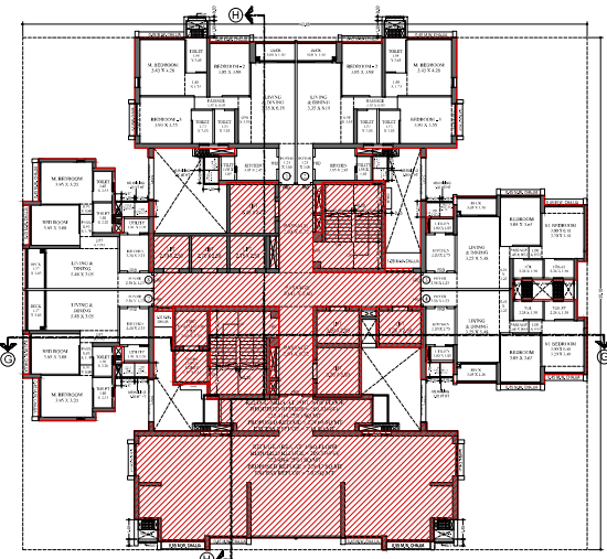
2ND, 3TH & 4TH TYPICAL REFUGE FLOOR PLAN (WING-4)
