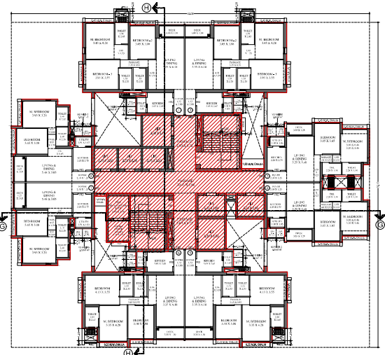
30TH TO 35TH, 37TH TO 42ND, 44TH TO 47TH TYPICAL FLOOR PLAN (WING-4)
