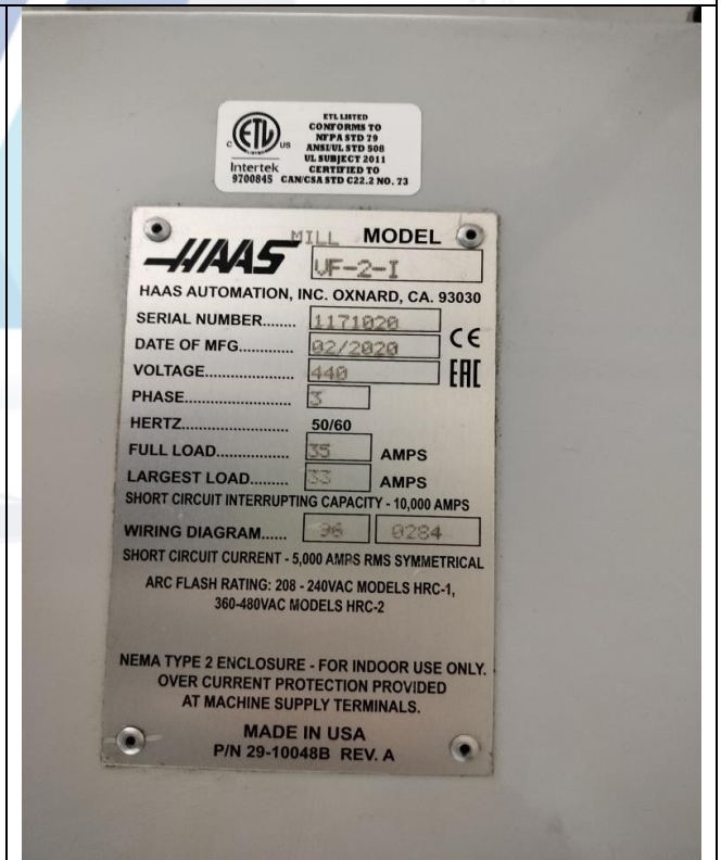
VF-2-I Vertical Machining Centre, Sr. No. 1171020
