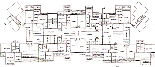
SANCTIONED PLAN AS PER CODE: CODE NO. 15181/TROMM & K/2017/7040 25 May 2018 TYPICAL - 7, 13 FLOOR PLAN
