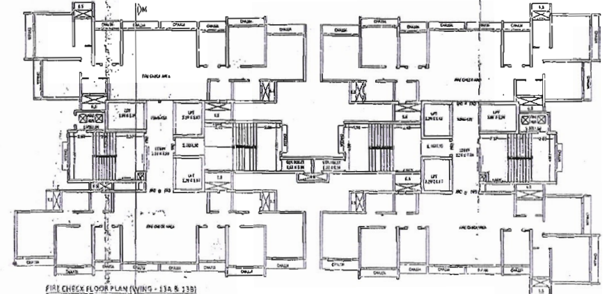
FIRE CHECK FLOOR PLAN (WING - 13A & 13B) SCALE - 1:100
