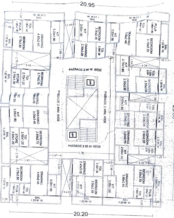
FIFTH FLOOR PLAN
