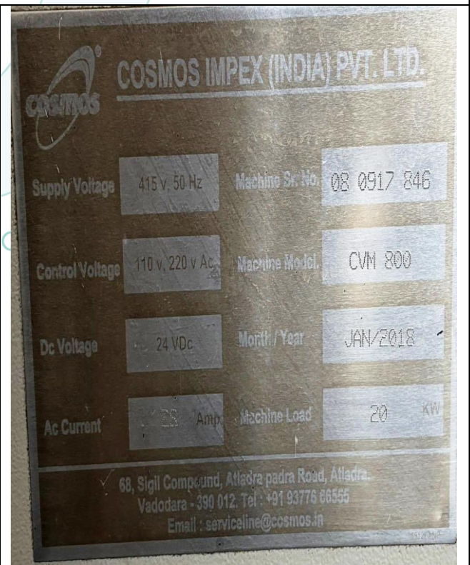
Used Cosmos make CNC Vertical Machining Centre, Model-CVM-800 with Siemens 828D CNC Controller ATC and other machine features, Sr. No. 08 0917 846, YOM-01/2018
