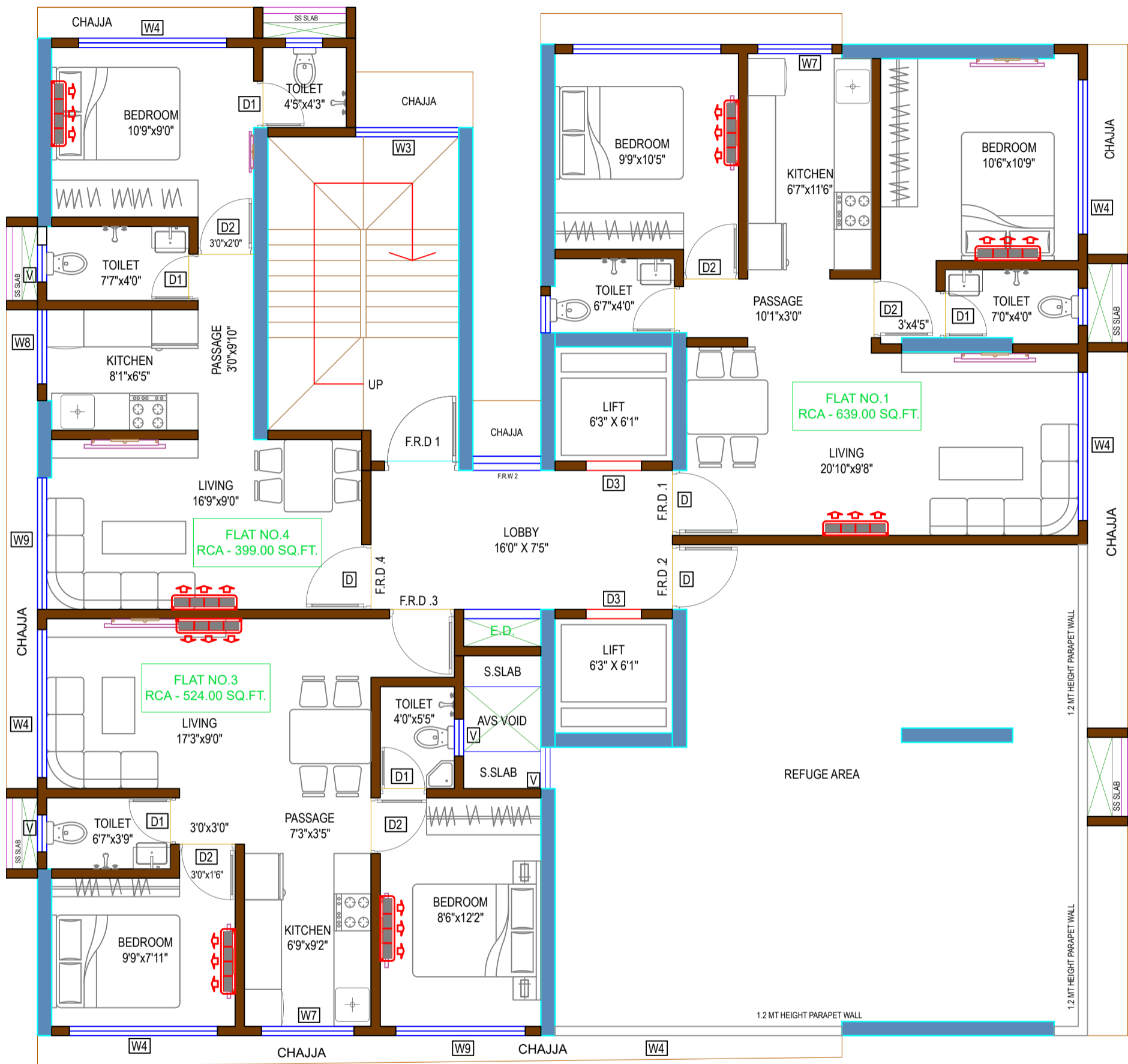
13TH FLOOR PLAN (REFUGE) SCALE 1:100
