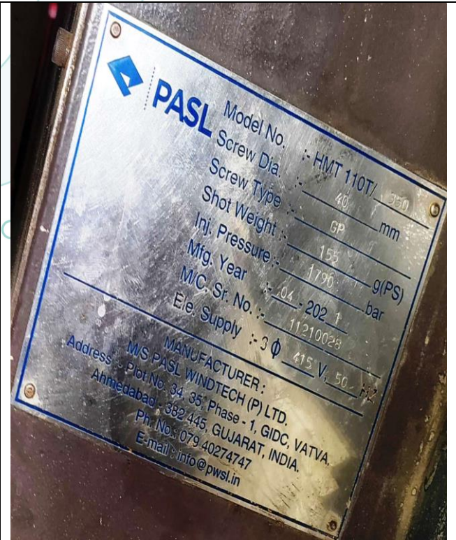
Fully Automatic Microprocessor Control Plastic Injection Moulding Machine with Servo, Model- HMT 110 T/ 350, Sr. No. 11210028
