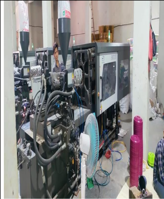
Fully Automatic Microprocessor Control Plastic Injection Moulding Machine with Servo, Model- HMT 110 T/ 350, Sr. No. 11210032
