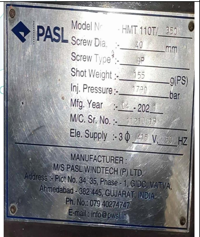
Fully Automatic Microprocessor Control Plastic Injection Moulding Machine with Servo, Model- HMT 110 T/ 350, Sr. No. 11210019
