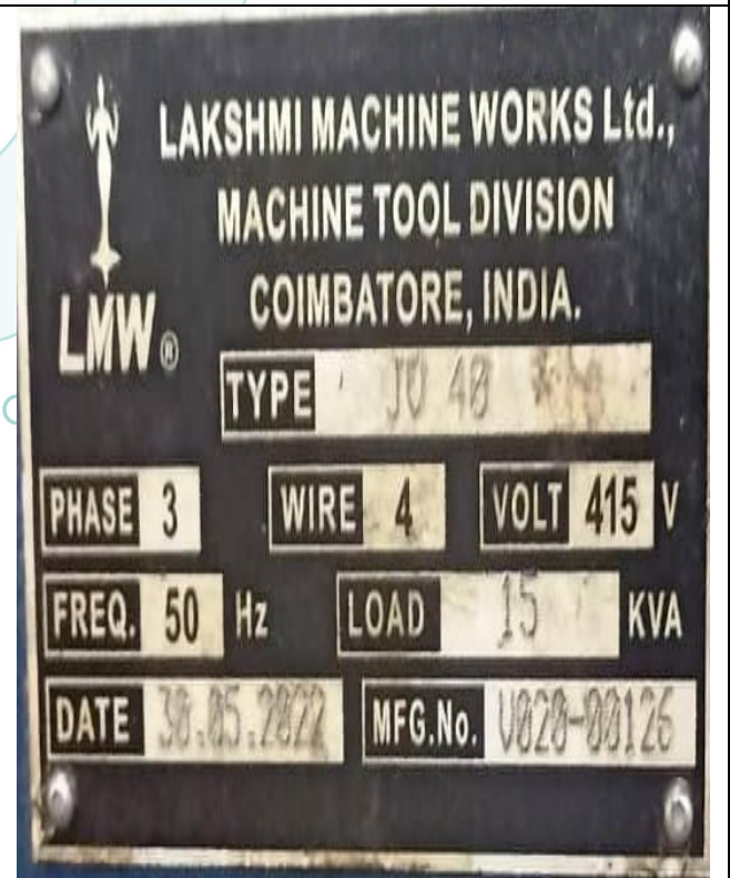
JV 40 CNC Vertical Machining Centre-Fanuc, Sr. No. V020-00126
