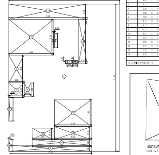
2ND TO 3RD FLOOR AREA DIAGRAM SCALE=1/100
