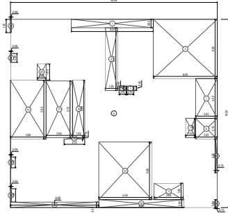
1ST TO 3RD FLOOR AREA DIAGRAM SCALE=1/100
