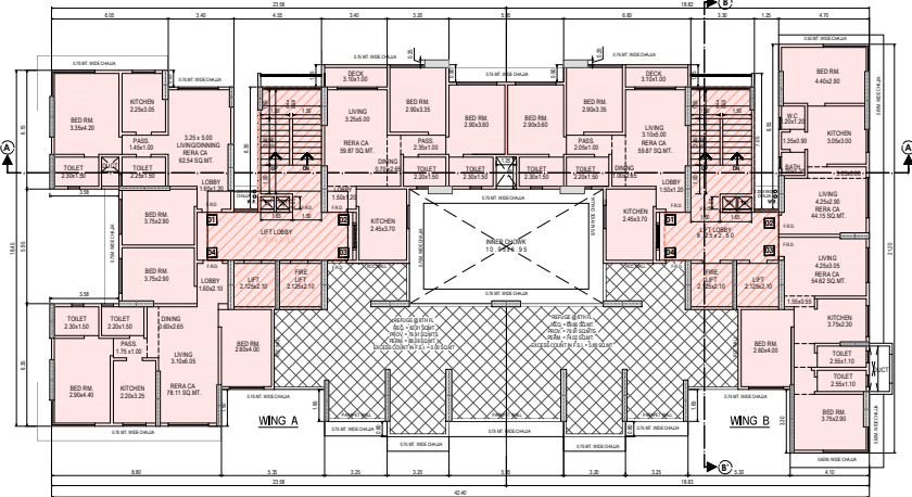
REFUGE FLOOR PLAN 8TH FLOOR SCALE: 1:100
