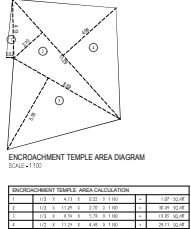
ENCROACHMENT TEMPLE AREA DIAGRAM SCALE=1/100
