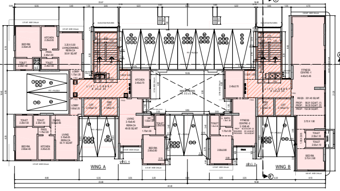
FIRST FLOOR PLAN SCALE=1/100
